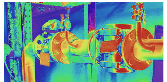
Typical sector valve thermal non-uniformity
